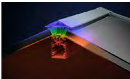
28mm glazing units with 1.0 Wm²K U-Value
